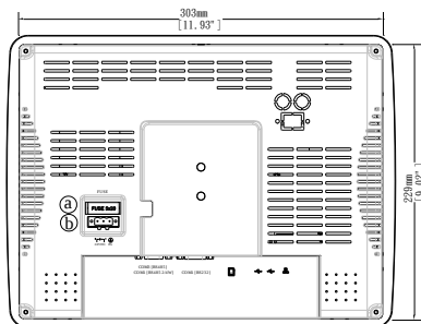
Rear View
