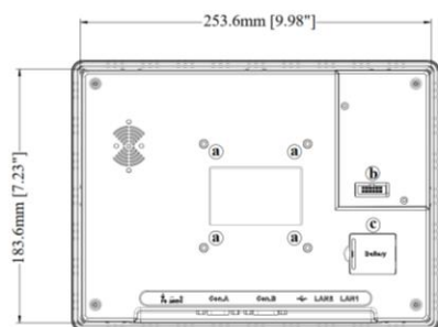
Rear View
