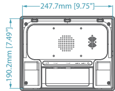
Rear View
